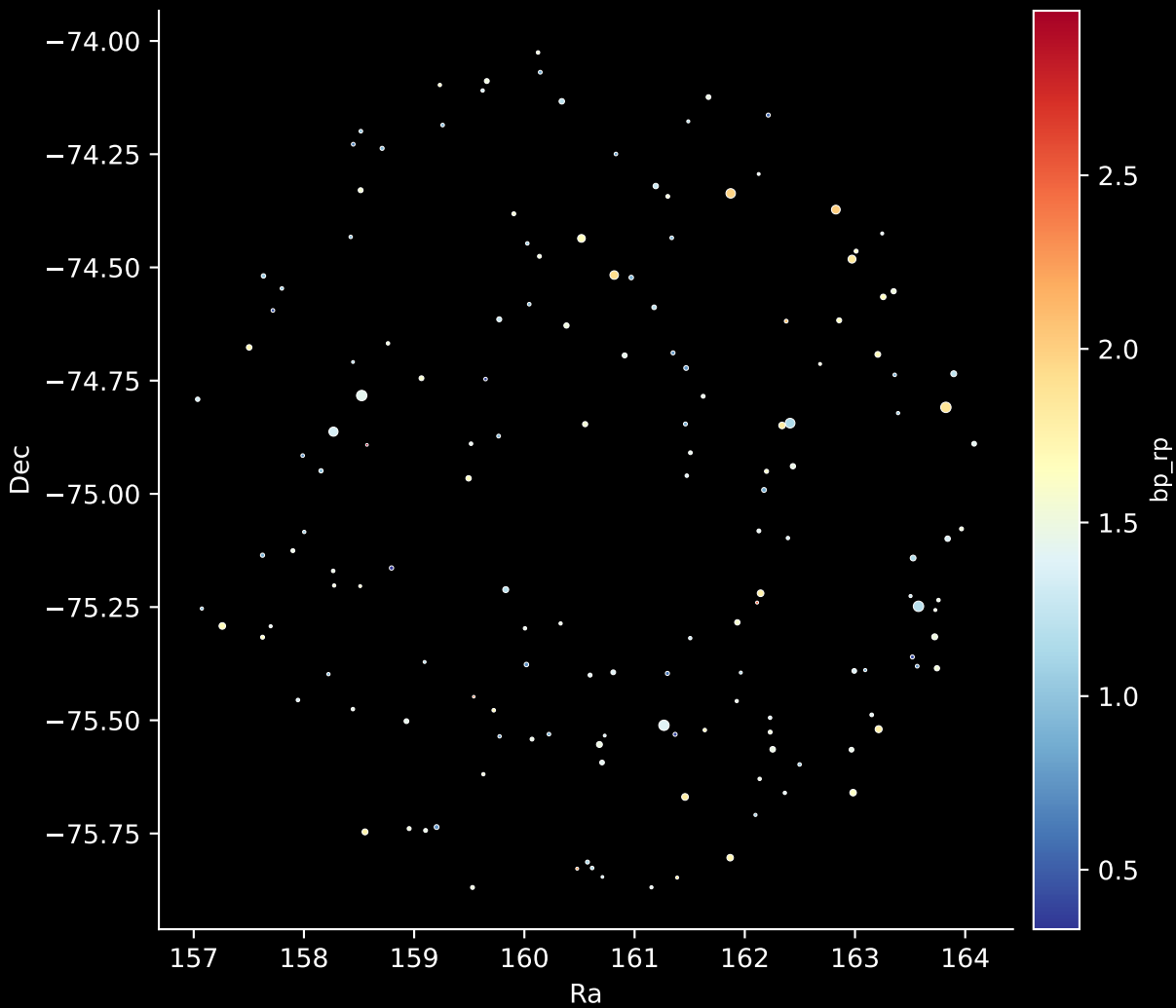
APOGEE DR17 Field: [LMC35] Stars: 156
