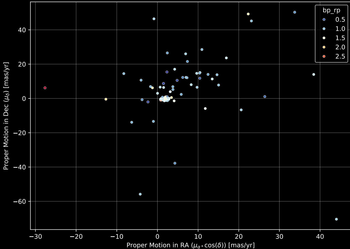
APOGEE DR17 Field: [LMC35] Proper Motion Diagram (n= 156)
