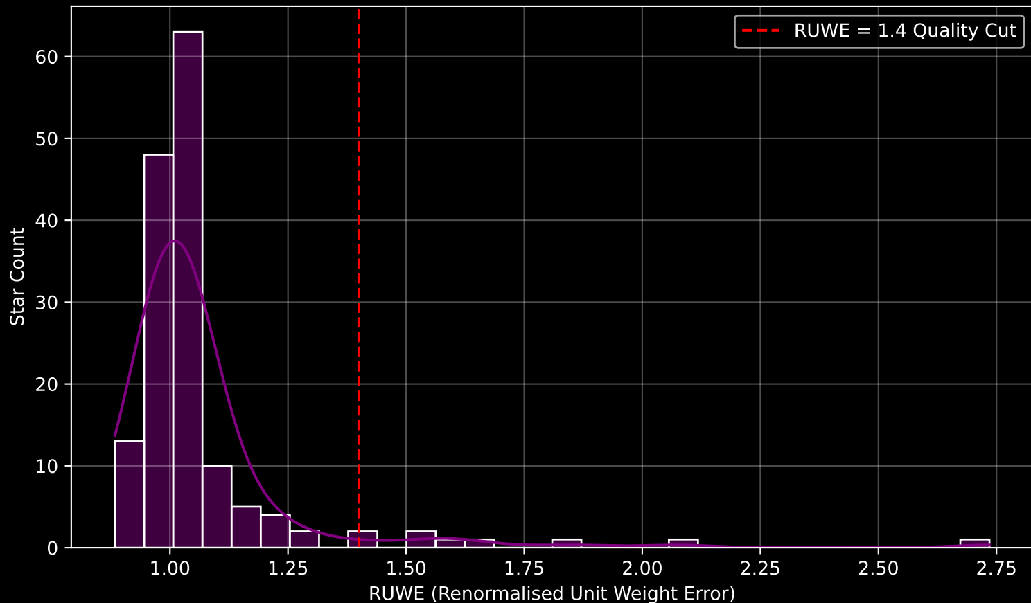
GAPOGEE DR17 Field [LMC35] RUWE Distribution (n= 154)
