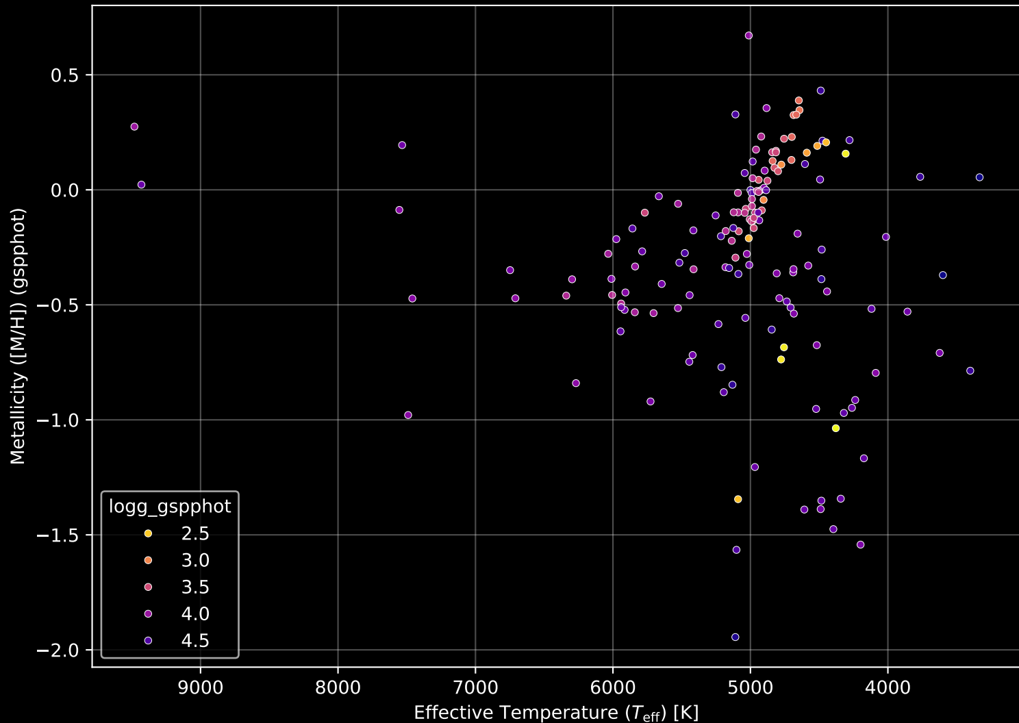
APOGEE DR17 Field: [LMC35] Stellar Population Parameters (n= 156)
