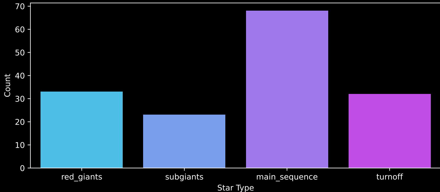
APOGEE DR17 Field: [LMC35] Count plot of Star Type
