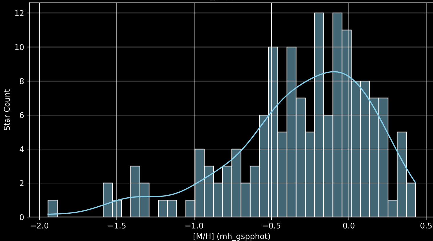
APOGEE DR17 Field: [LMC35 [M/H] (mh_gspphot) (n= 155)
