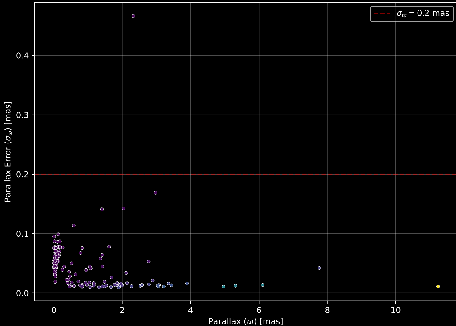
APOGEE DR17 Field: [LMC35] Parallax Quality (n= 156)
