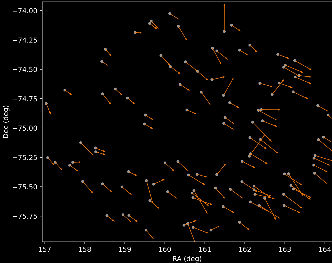
APOGEE DR17 Cluster 2 Proper Motion Vectors (n=107)
